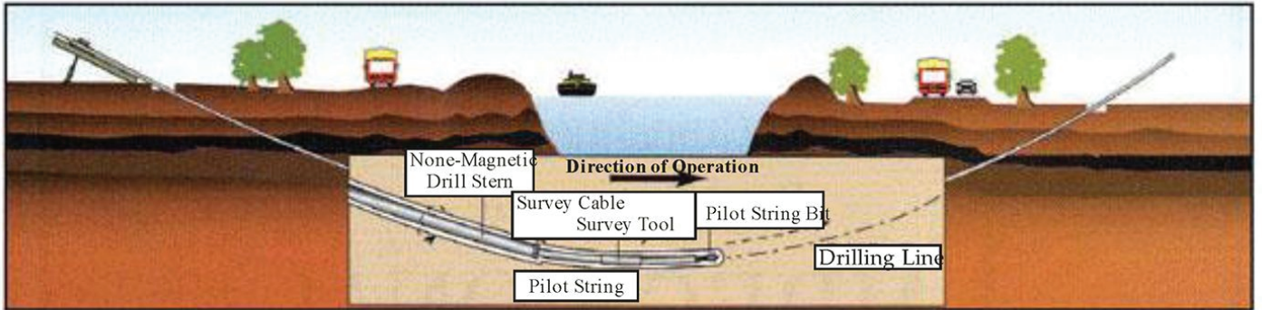
Pilot drilling
