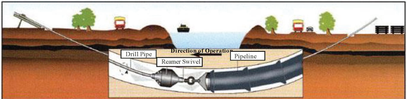
Installation of the carrier pipe
