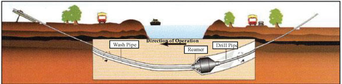
Drilling diameter expansion
